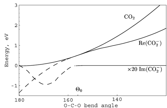
FIG. 1. Cuts through the potential surfaces of \text{CO}_2 and \text{CO}_2^- where the O-C-O angle \Theta , in degrees, is varied and the C-O bond distance is fixed at 2.2 bohrs. In the crossing region, around \Theta_o , the difference between the curves follows a threshold law predicted by the dipole moment of \text{CO}_2 . This law allows us to analytically continue the \text{CO}_2^- potential into configurations where it is unbound, denoted by dashed curves, and construct a complete surface for the \text{CO}_2^- virtual state.
