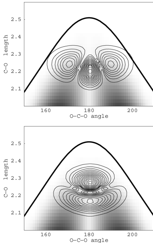
FIG. 3. Contour plots of the wave functions for the two components of the Fermi dyad in O-C-O angle, in degrees, and C-O bond distance, in bohrs. The thick line marks the seam where the anion and neutral surfaces cross. The imaginary part of the anion surface is zero above the seam and increases proportionately in regions indicated by the shading. Top panel: upper member of dyad; bottom panel: lower member of dyad.
