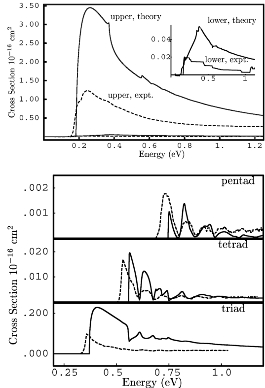
FIG. 2. Excitation cross sections for the Fermi polyads in \text{CO}_2 . Solid lines: theory; dashed lines: experiment (Refs. [5,6]). Top panel: dyad; bottom panel: triad, tetrad, and pentad.
